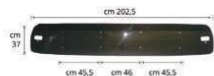
VISIERA PMMA COS.PEL. ref. 707.15300
