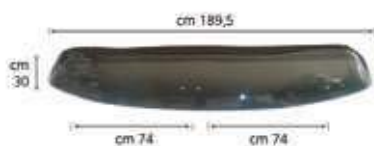
VISIERA PMMA COS.PEL. ref. 704.55100
